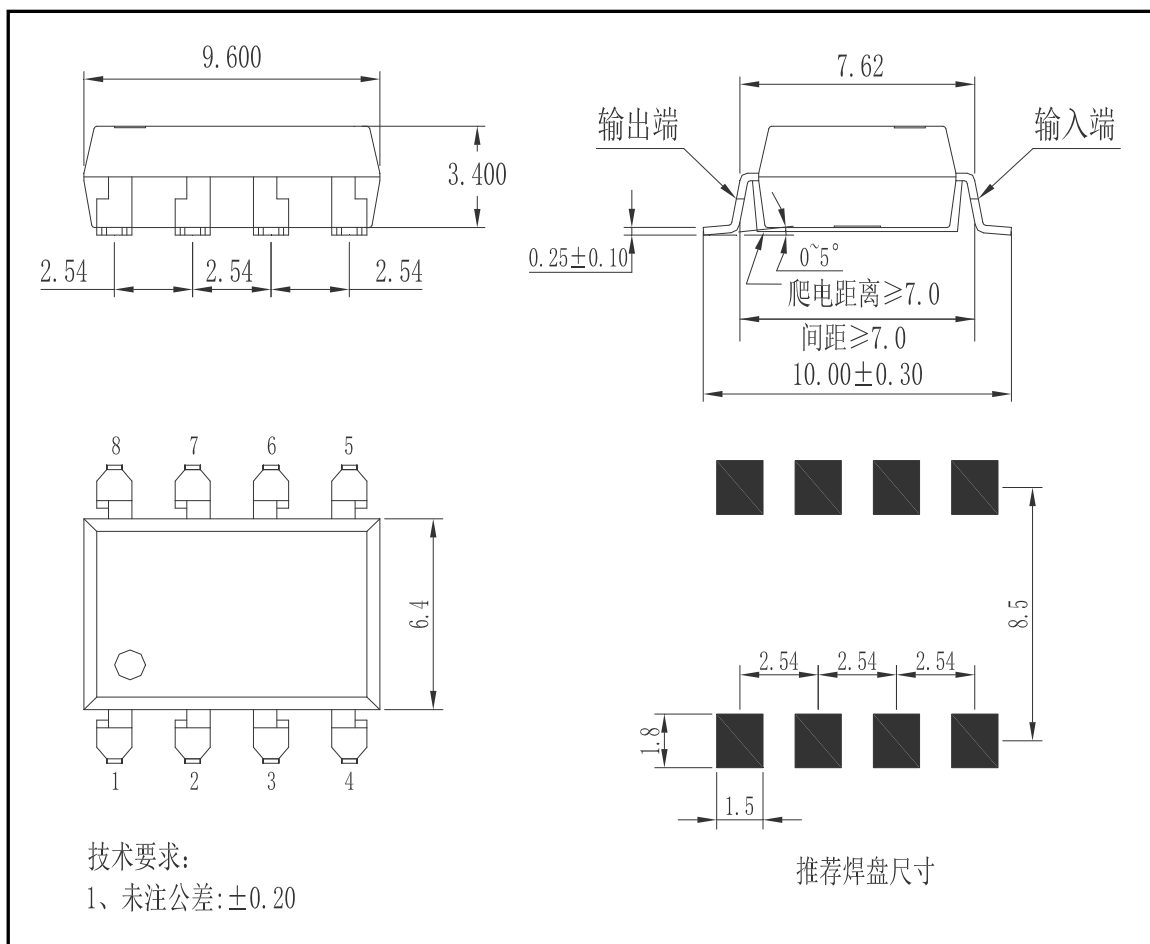
图 4 HSSR-DA08-2 外形尺寸 Figure 4- The dimensions of HSSR-DA08-2
