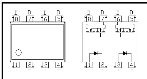
图 2 电原理图 Figure 2-Schematic
