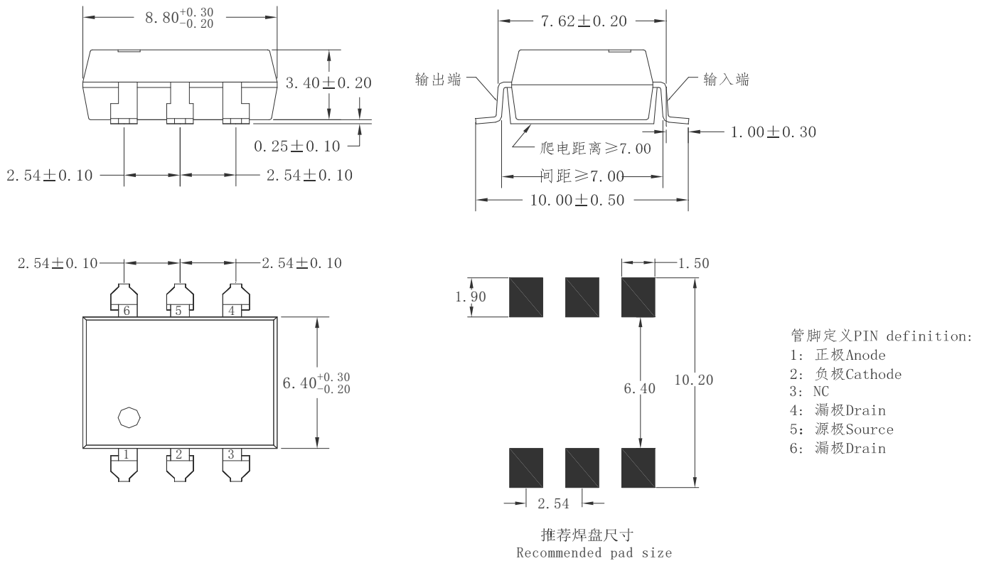
图 9 HSSR-61A09-2 外形尺寸 Figure 9- The dimensions of HSSR-61A09-2
