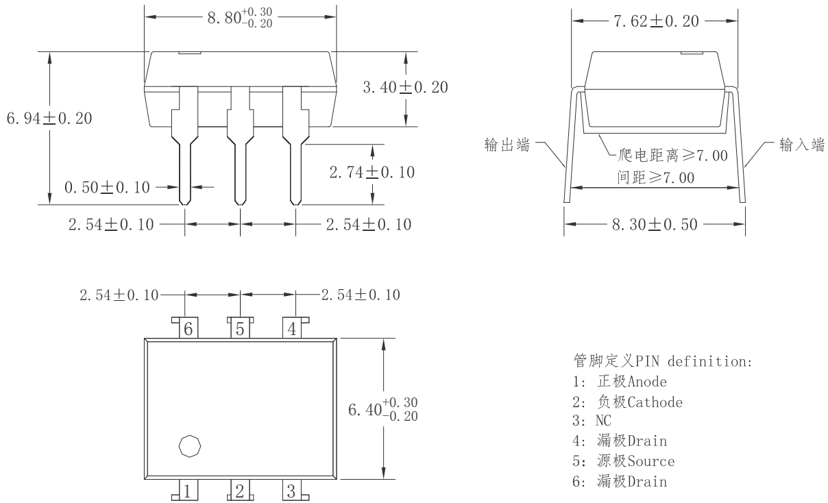
图 8 HSSR-61A09 外形尺寸 Figure 8- The dimensions of HSSR-61A09
