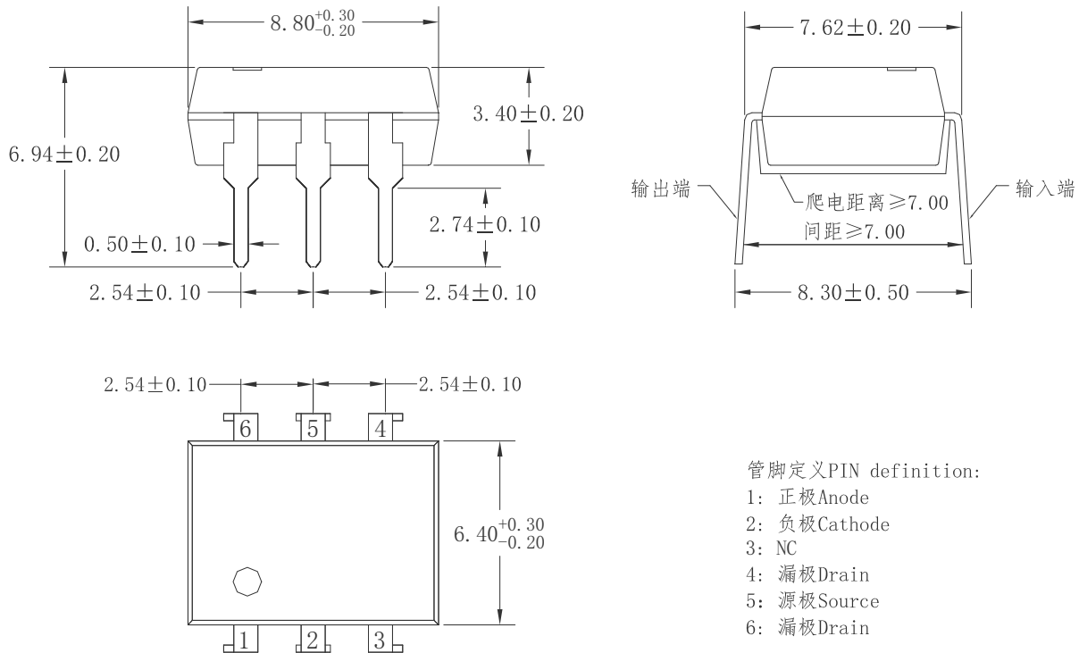
图 8 HSSR-61A05 外形尺寸 Figure 8- The dimensions of HSSR-61A05
