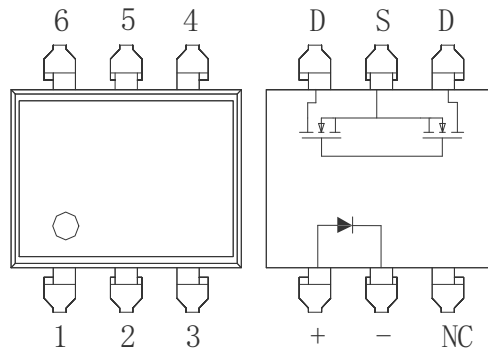
图 2 电原理图 Figure 2-Schematic
