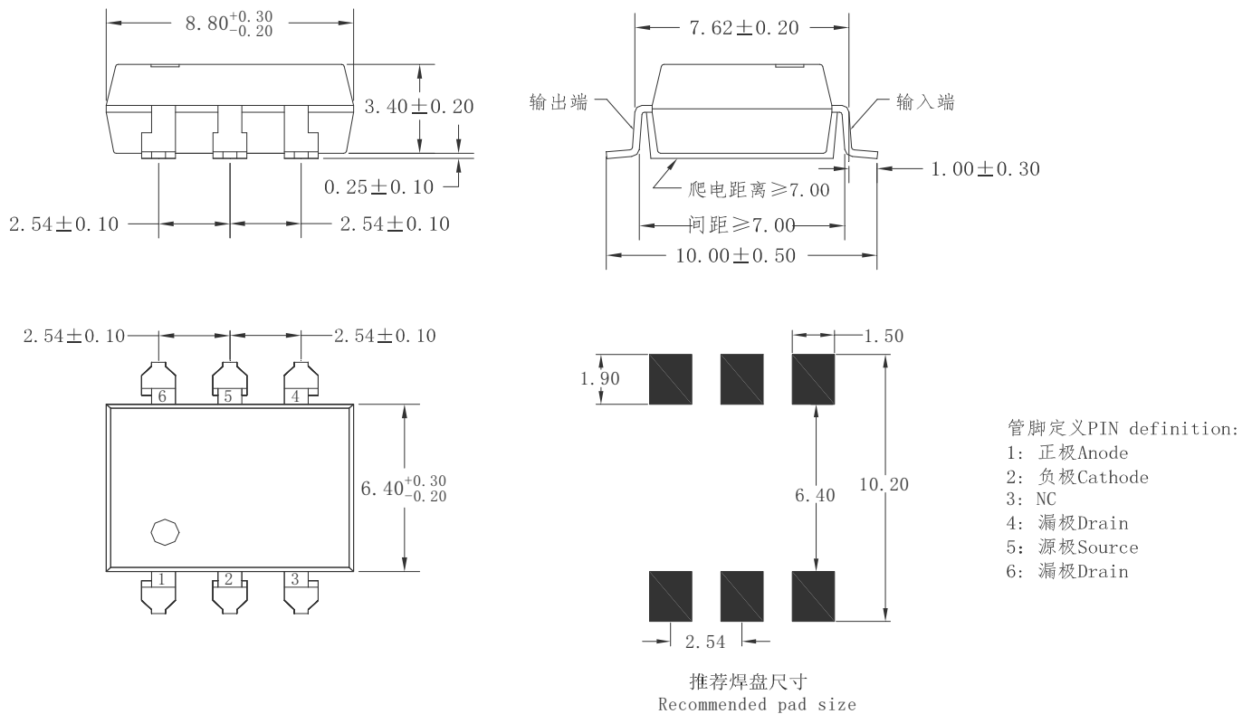
图 9 HSSR-61A05-2 外形尺寸 Figure 9- The dimensions of HSSR-61A05-2
