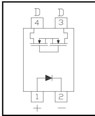
图 2 电原理图 Figure 2-Schematic
