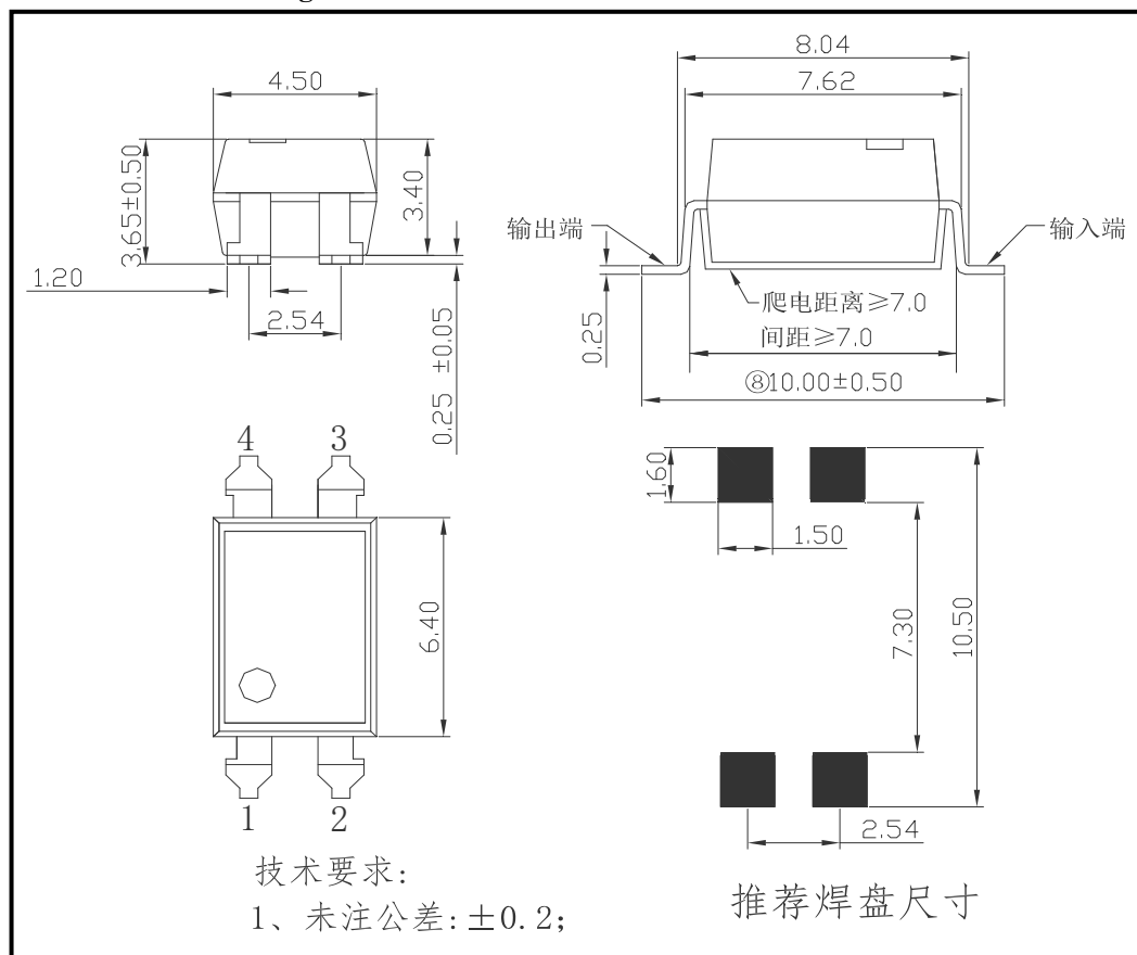
Figure 3- The dimensions of HSSR-41A11
